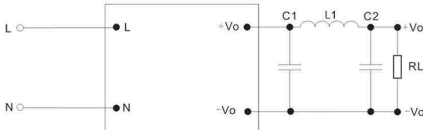
Circuit 2
